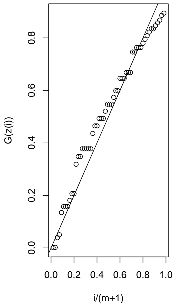
Probability plot
