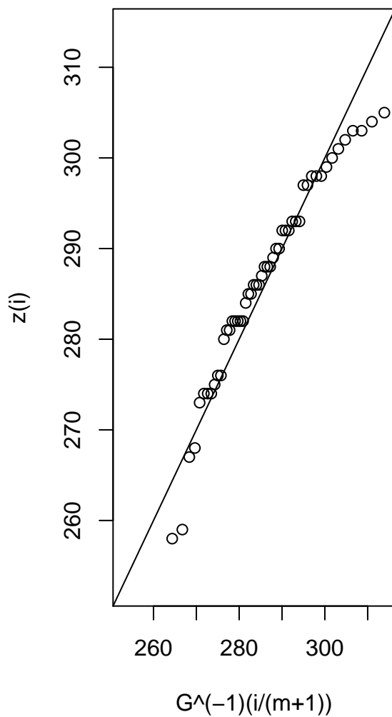
Quantile plot
