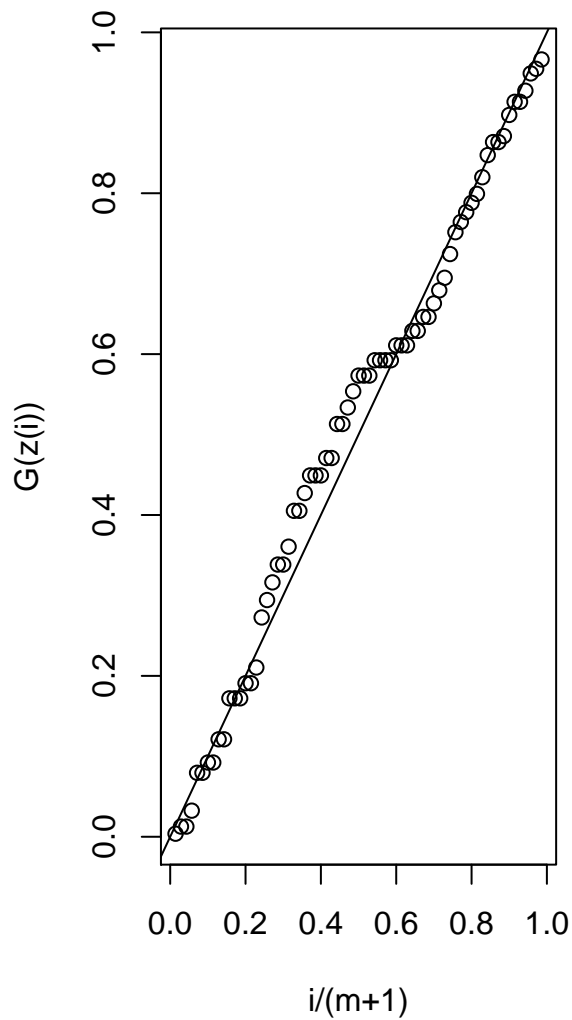
Probability plot
