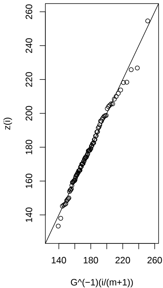
Quantile plot
