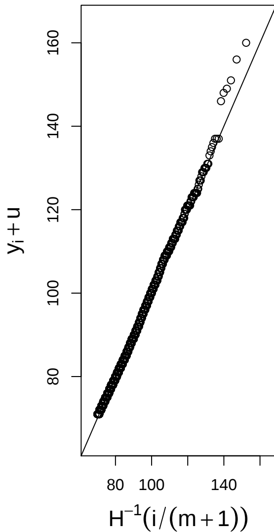
Quantile plot
