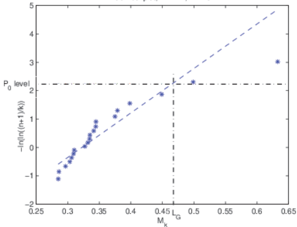
Gumbel plot, H=12m, T=12s
