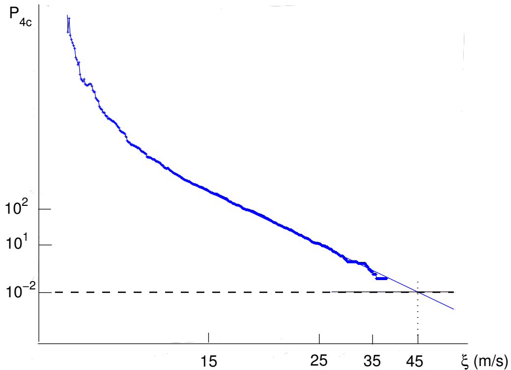
Transf plot of 4th cond. cascade
