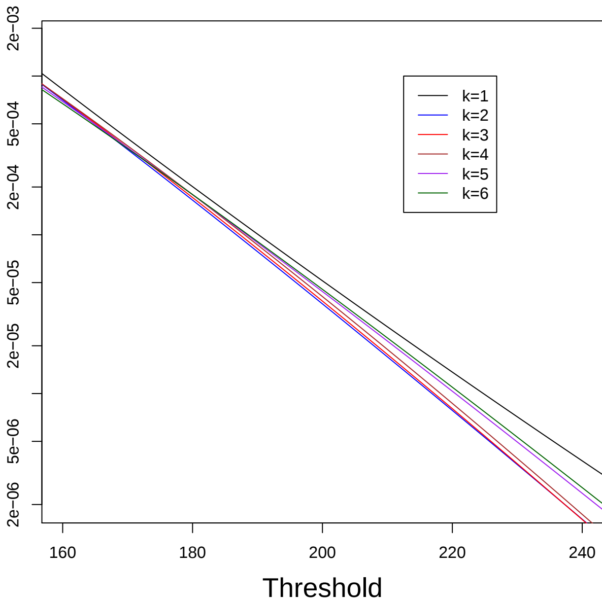
Estimated ACER functions for high levels in Viker
