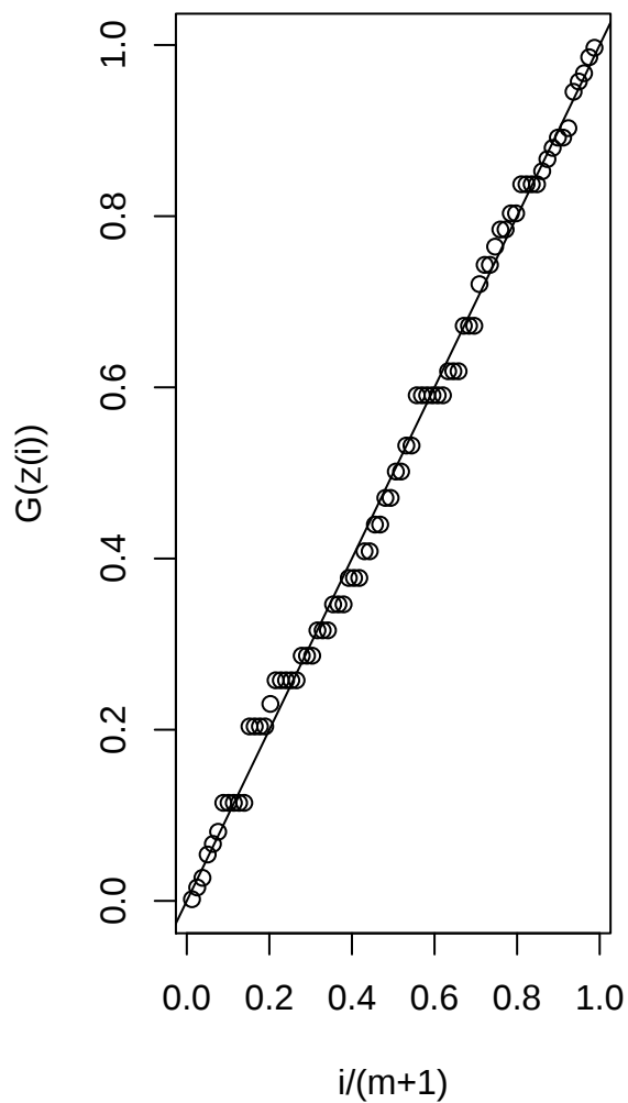
Probability plot
