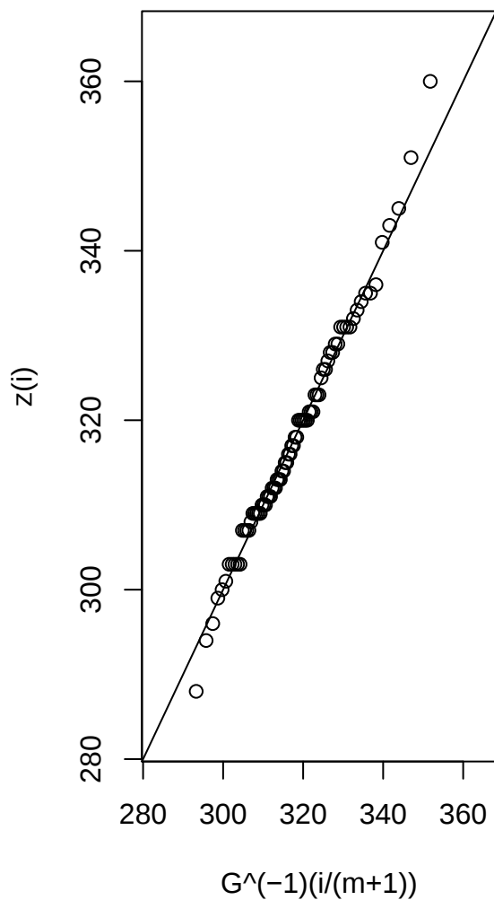
Quantile plot
