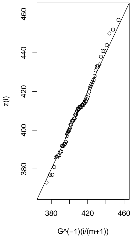
Quantile plot
