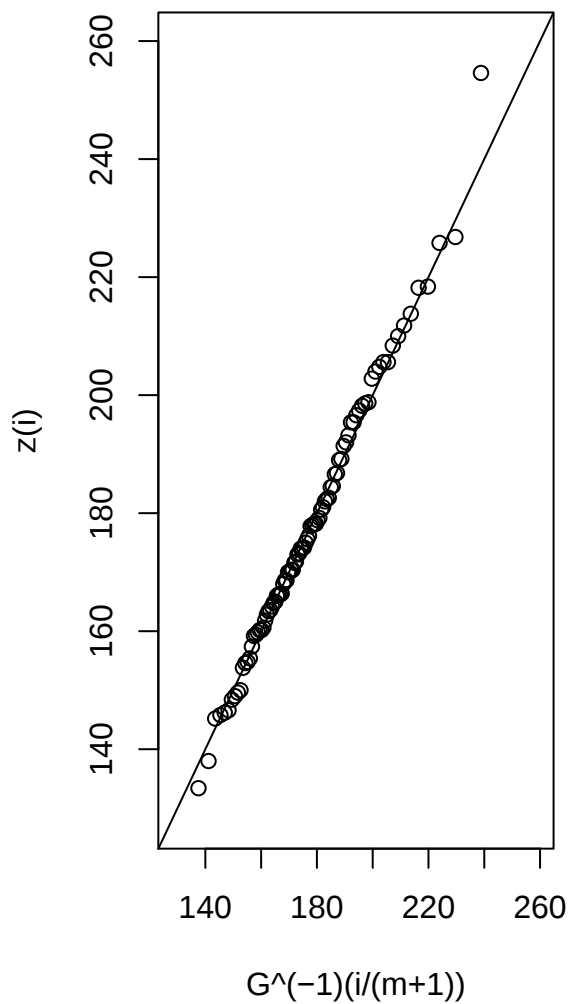
Quantile plot
