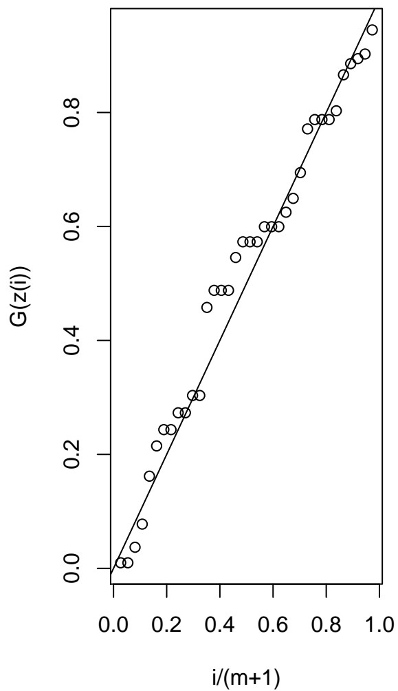
Probability plot
