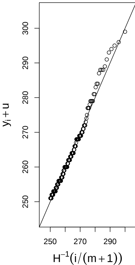
Quantile plot
