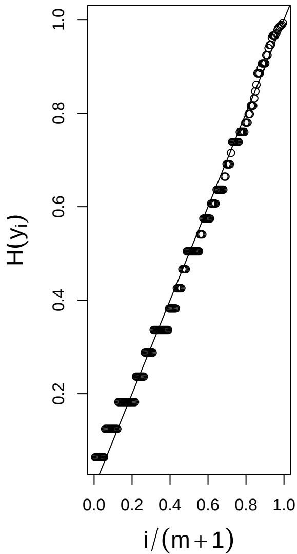
Probability plot
