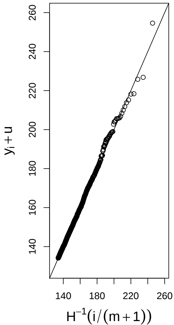
Quantile plot
