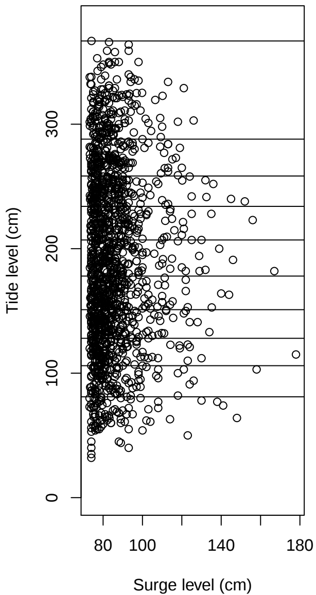
Surge data
