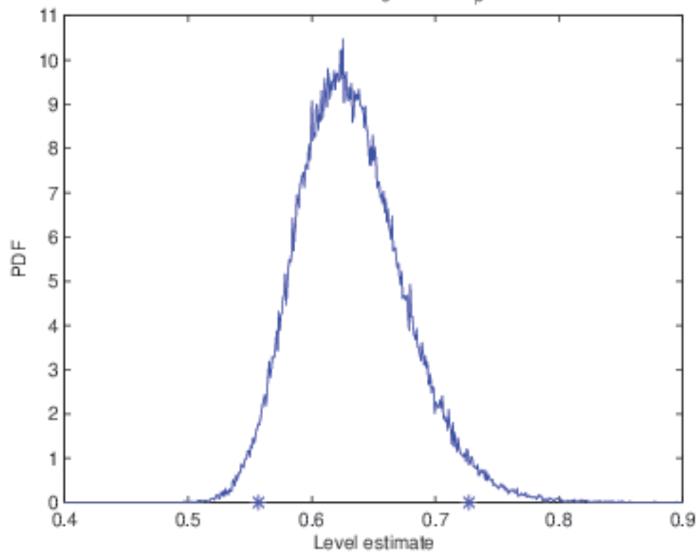
Bootstrapped PDF, H_s=14.7\text{m} , T_p=16.5\text{s}
