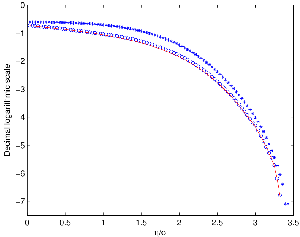
Duffing oscillator \zeta=4\% , \lambda=0.5
