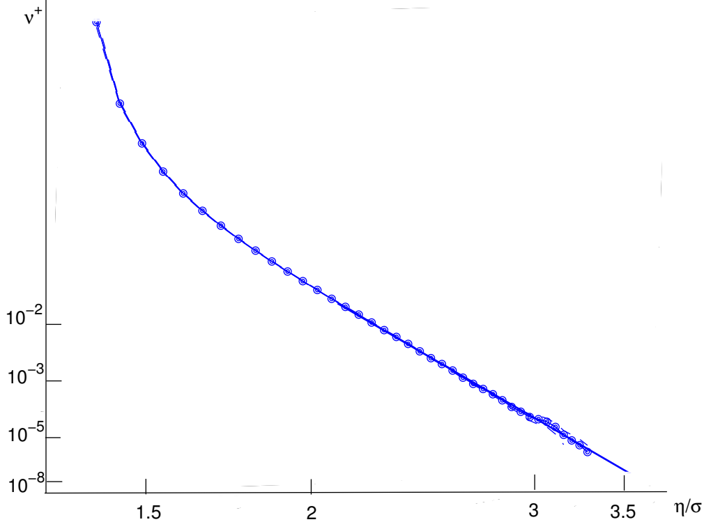
Transformed plot: Duffing, \zeta=2\% , \lambda=5
